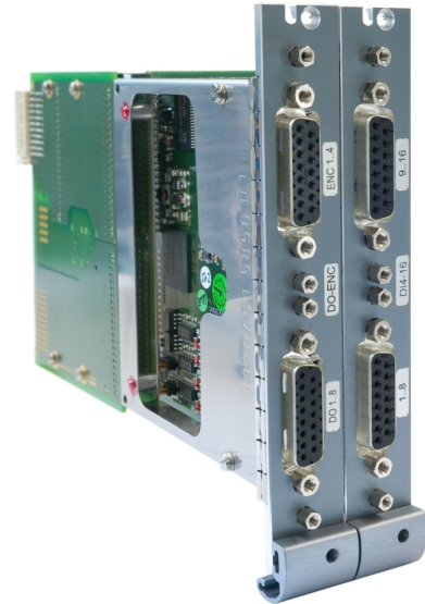
Fig. similar CRC/DI8-DO8-ENC4-DAC4
